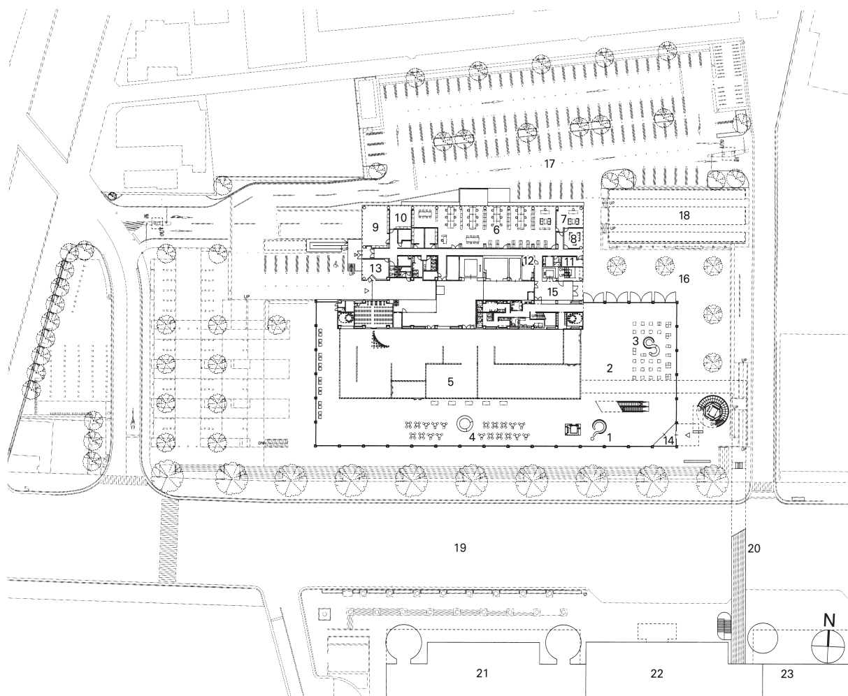
1F Plan
